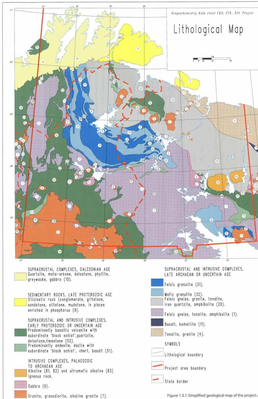
Figure 1.3.1: Simplified geological map of the project area.
